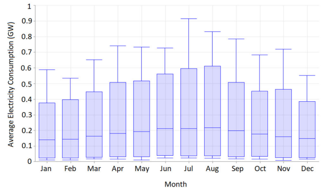
Fig. 3. Monthly profile of residential electricity demand in Yazd city by combining accurate weather data and the standard profile of electricity demand in HOMER.
