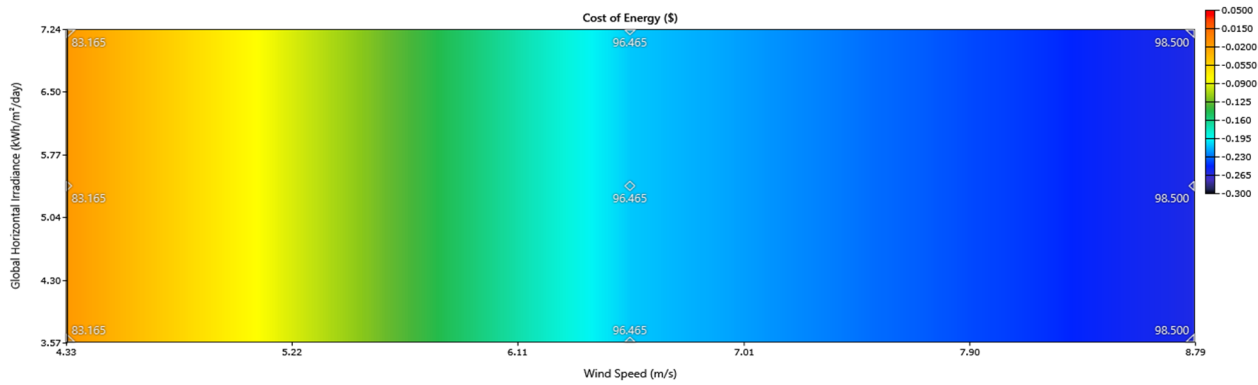
Fig. 8. Sensitivity of Cost of Energy based on the Wind Speed (x-axis) and Global Horizontal Irradiance (y-axis). Inside numbers show Renewable Fraction.
