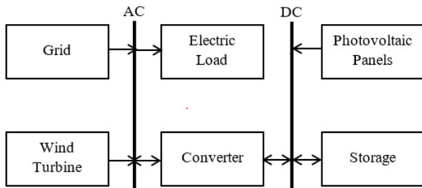
Fig. 2. The diagram of the investigated RES.
