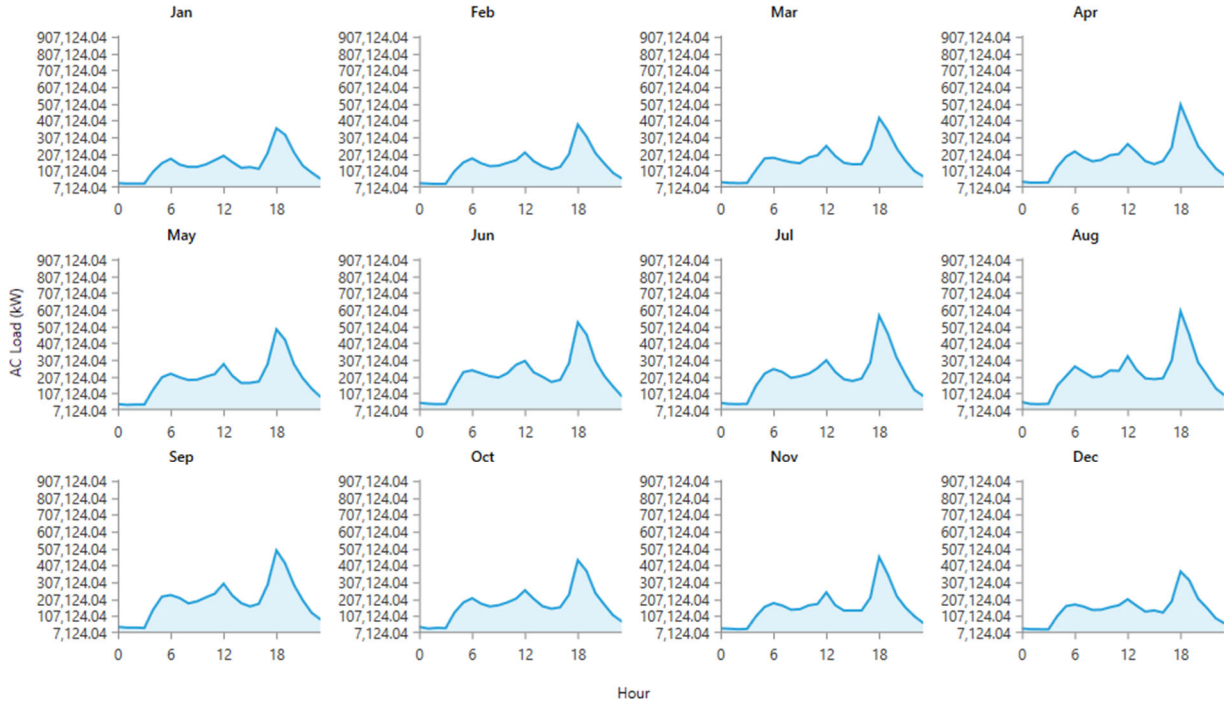
Fig. 5. Monthly profile of AC load in the study area by combining accurate weather data and the standard profile of electricity demand in HOMER.
