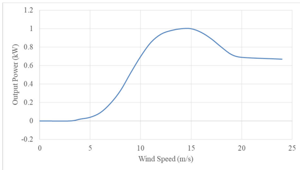
Fig. 4. The output power curve of the considered wind turbine for Yazdi city [83, 84].
