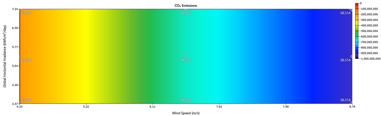
Fig. 9. Sensitivity of CO 2 Emission based on the Wind Speed (x-axis) and Global Horizontal Irradiance (y-axis). Inside numbers show Renewable Fraction.
